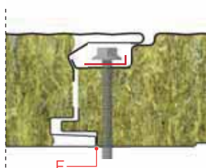
Joint detail
