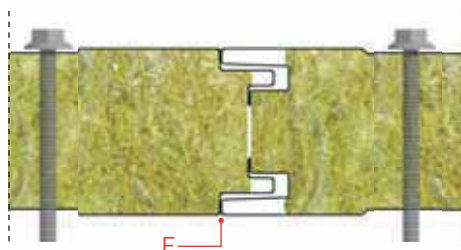
Joint detail
