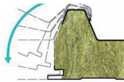
Details of the assembly phase
