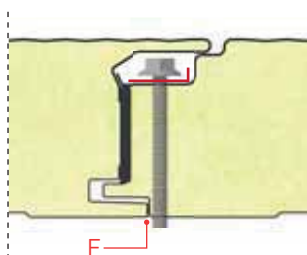
Joint detail
