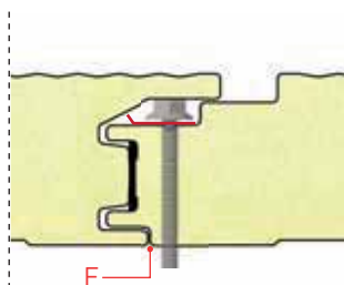
Joint detail
